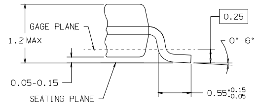
DETAIL A TYPICAL
